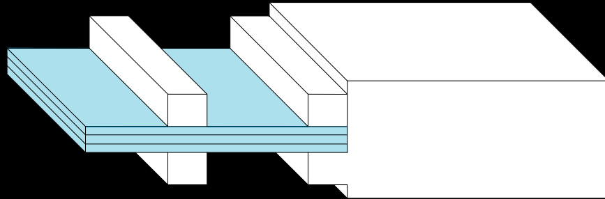
SQUARE MUNTINS (SDL) - EXTERIOR SQUARE STICKING
