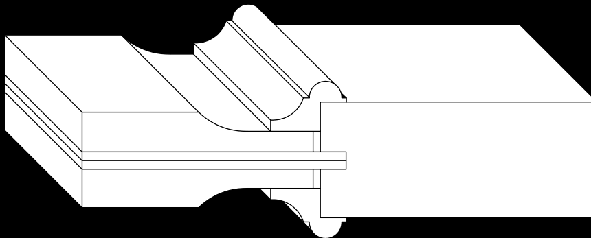
SCOOP RAISED PANEL - V15 INSET BOLECTION MOULDING
