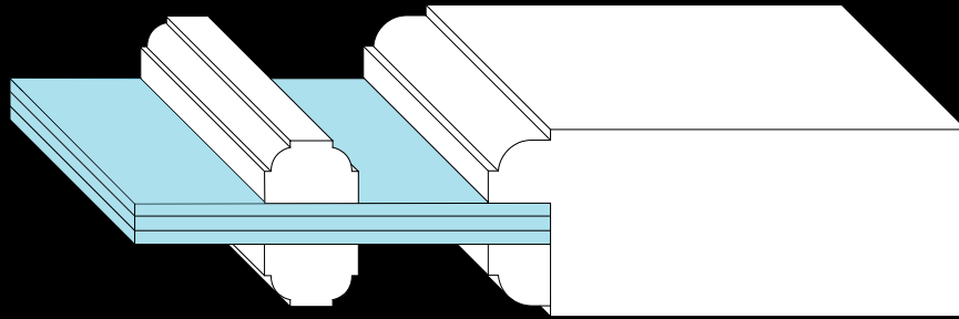
OVOLO MUNTINS (SDL) - EXTERIOR OVOLO STICKING (STANDARD)
