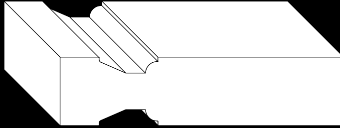
BEVEL PANEL / QUARTER BEAD STICKING (STANDARD)
